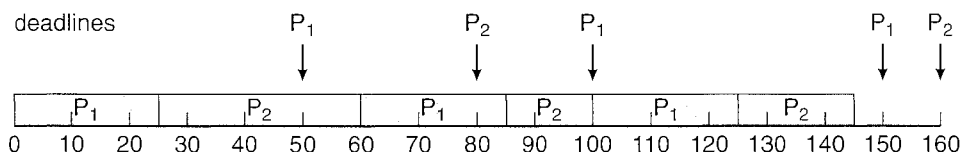
Figure 19.10 Earliest-deadline-first scheduling.
